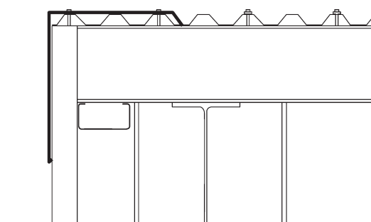
Typical Barge Capping
