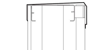
Typical Parapet Capping
