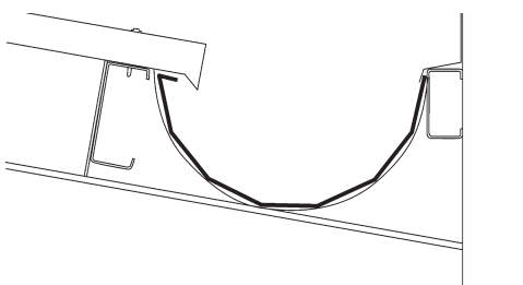
Typical Trough Gutter
