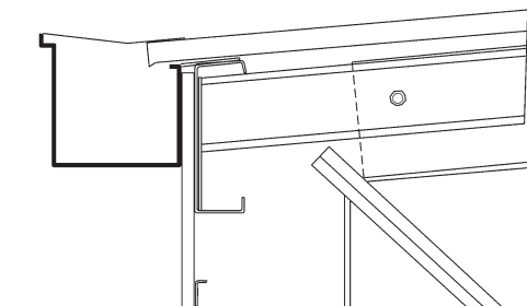
Typical Eaves Gutter
