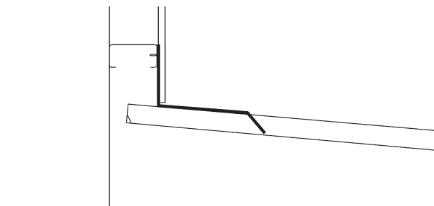
Typical Apron Flashings
