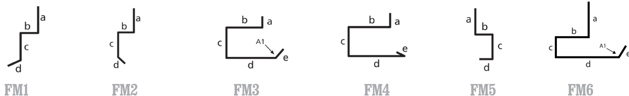
Typical Foot Mould
