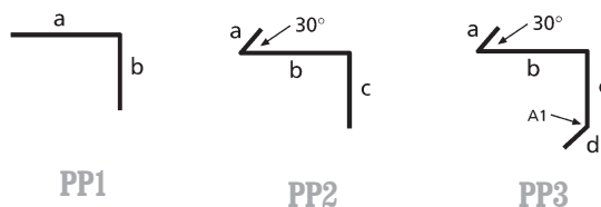
POLE PLATE FLASHING
