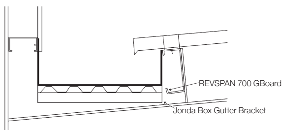
Typical Box Gutter
