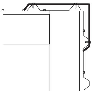
Typical Corner Flashing
