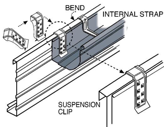
115 QUAD - STEEL FASCIA
