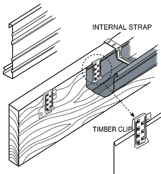
115 QUAD TIMBER OR STEEL FASCIA
